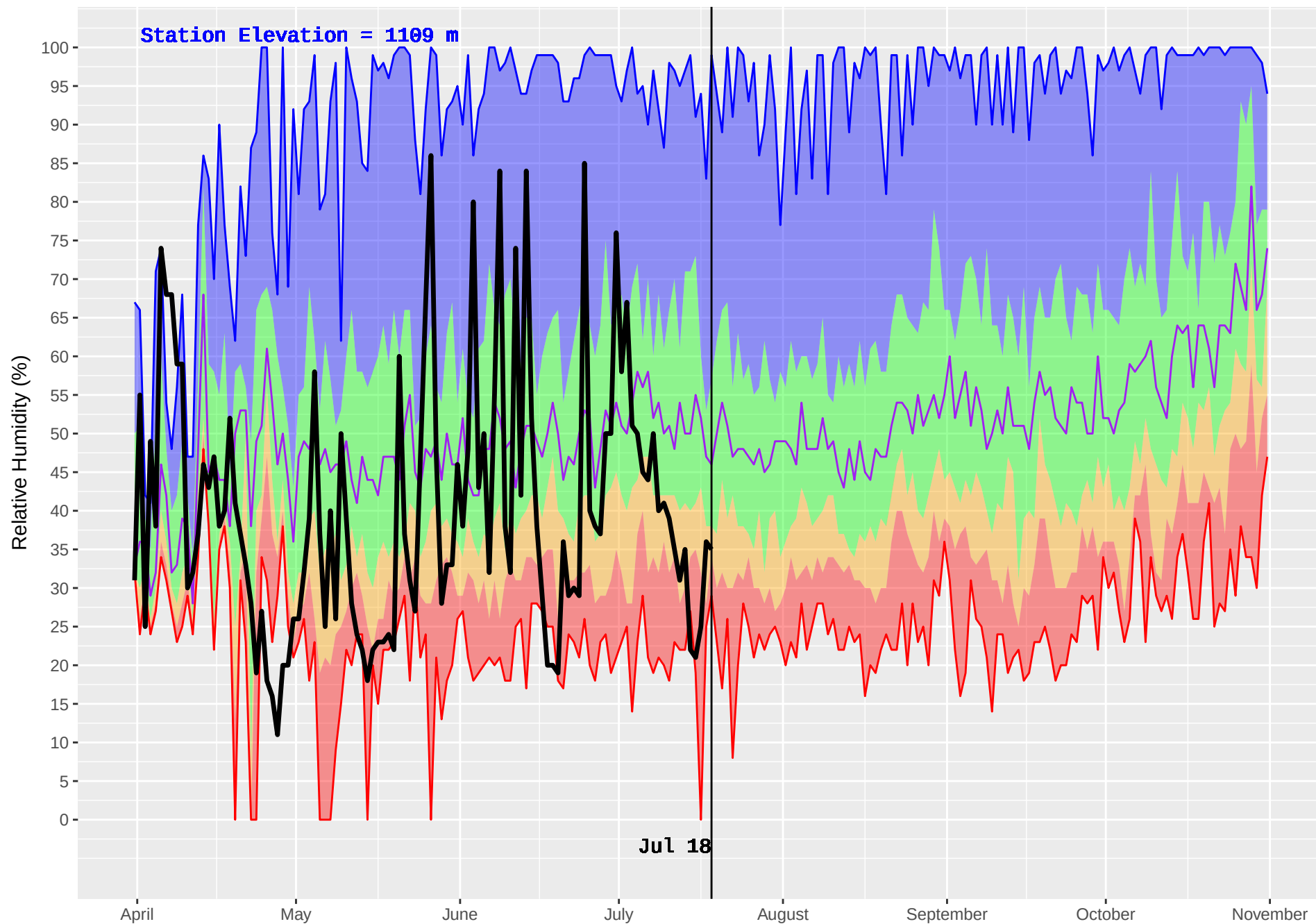
MOOSE LAKE (165) : Historical (1980–2016) and Current (2018) Daily Relative Humidity
